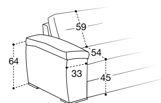
SPALLIERA IN FIOCCO BACK WITH FLOCK DOSSIER EN FLOCON SEDUTA IN POLIURETANO ESPANSO SITTING POLYURETHANE FOAM ASSISE MOUSSE DE POLYURETHANE
